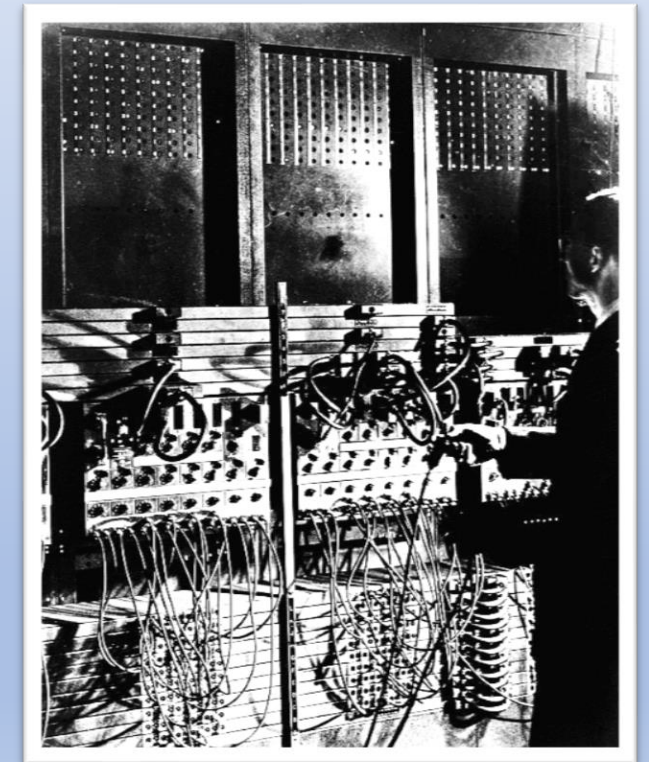
Two ENIAC accumulators Year: 1946 ca
